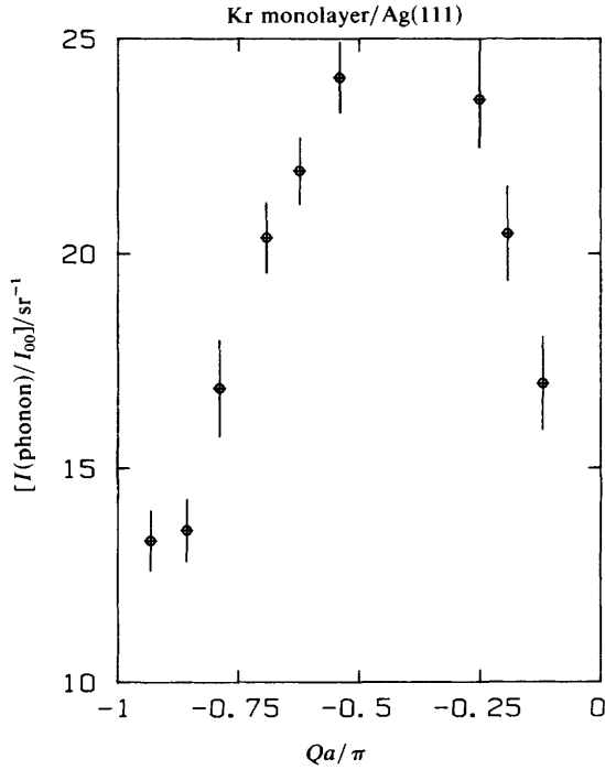
Fig. 8. Inelastic transition probabilities of 18 meV He scattering from a 25 K Kr monolayer, \theta_i = 45^\circ . Data are for momentum loss (with respect to the beam), in the first surface Brillouin zone, of the lowest-energy transition corresponding to phonon creation. This is the largest feature in fig. 7.
