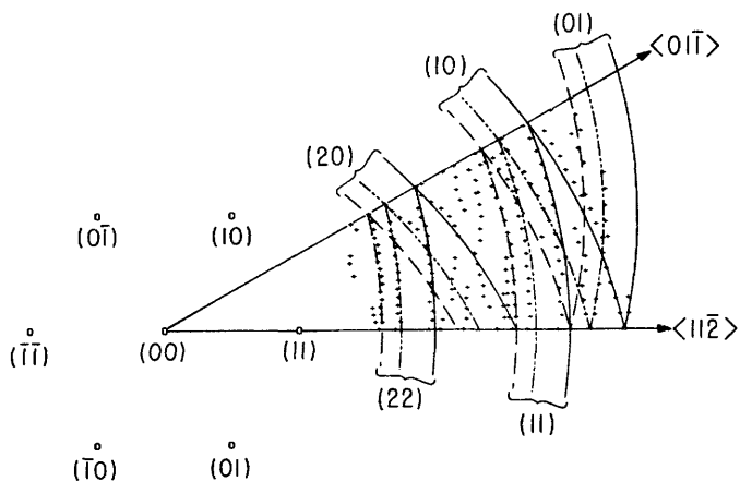
Fig. 3. K_x - K_y plot of the specular intensity maxima which occurred in the selective adsorption experiments for the Xe monolayer, using an 18 meV He beam. The specular intensity was monitored at 0.2^\circ increments of polar angle for a fixed crystal azimuth, from approximately 25 to 75^\circ . This was repeated for every 2^\circ of azimuth from the \langle 11\bar{2} \rangle to the \langle 01\bar{1} \rangle directions. Arcs are drawn for three energy levels, assuming the free-atom approximation, and are labelled with the coupling G vector (see text). T_s = 25 K.
