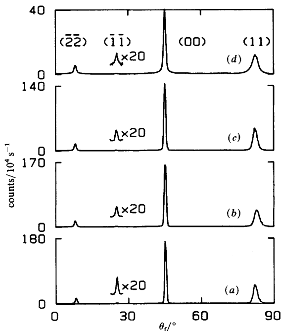
Fig. 1. Diffraction spectra for Xe overlayers physisorbed on Ag(111), taken in the \langle 11\bar{2} \rangle direction; with \theta_i = 45^\circ , T_s = 25 K and an 18 meV He beam. (a) 1, (b) 2, (c) 3 and (d) 25 layers. Conditions for all of the spectra are similar, so intensities are comparable.
