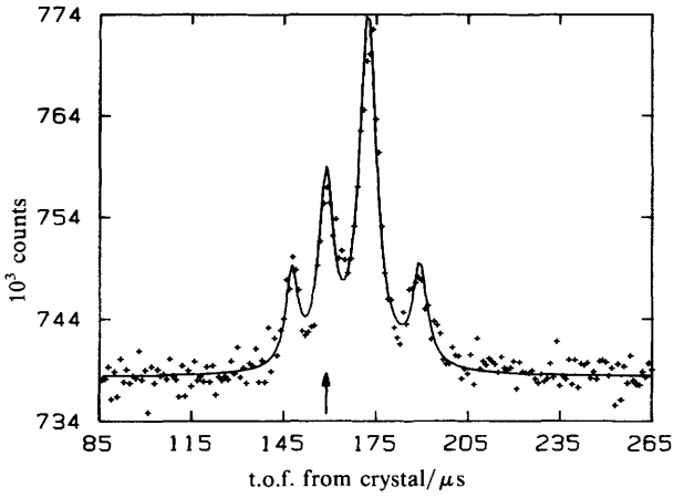
Fig. 7. Time-of-flight spectra for 18 meV He scattering from a Xe monolayer; \theta_i = 45^\circ , \theta_f = 47.9^\circ and T_s = 25 K. The arrow indicates the position of the elastic channel. Crosses are the experimental data, and the solid line is a forward convolution of the instrument function with the phonon dispersion curve, where the transitions are given a Lorentzian energy width.
