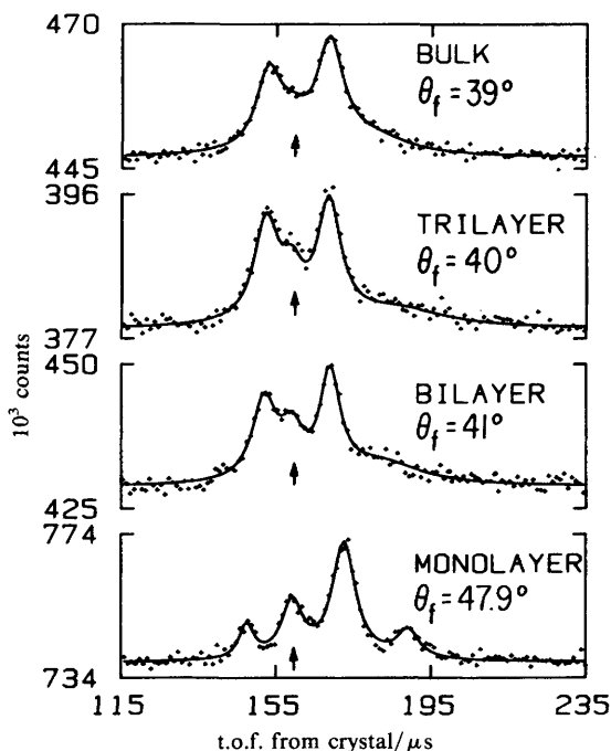
Fig. 4. T.o.f. spectra of Xe overlayers physisorbed on Ag(111); E_i = 18 meV, \theta_i = 45^\circ and T_s = 25 K. Crosses are the experimental data, and solid lines are a least-squares fit. (a) Monolayer, \theta_f = 47.9^\circ ; (b) bilayer, \theta_f = 41^\circ ; (c) trilayer, \theta_f = 40^\circ ; (d) bulk, \theta_f = 39^\circ .
