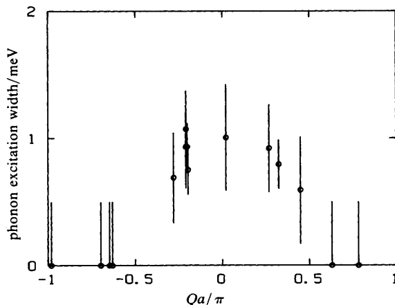
Fig. 9. Widths of the inelastic transitions for 18 meV He scattering from a 25 K Xe monolayer, \theta_i = 45^\circ . Data are for the lowest-energy transition corresponding to phonon creation.
