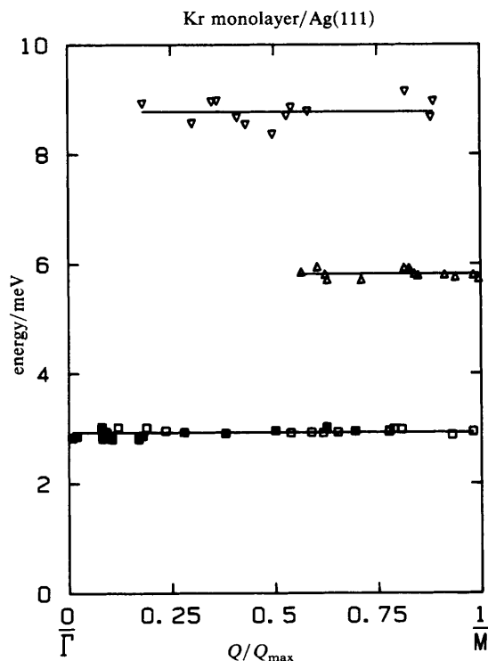
Fig. 6. Dispersion curves for Kr monolayer, showing the three observed frequencies. Open and closed symbols are the same as for fig. 5.
