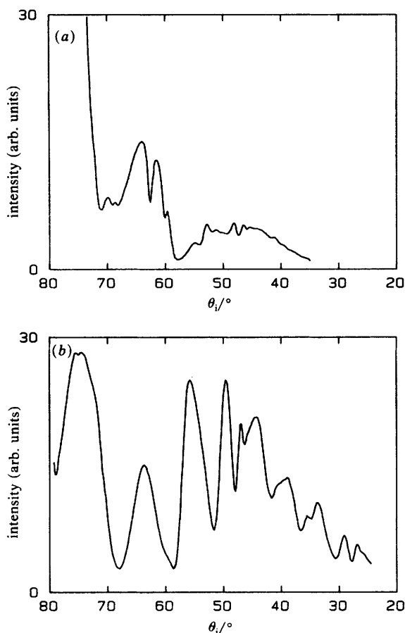
Fig. 2. Scans of the specular intensity for a Xe monolayer as a function of polar angle, with an He beam energy of (a) 66 and (b) 18 meV. Both selective adsorption spectra were taken in the \langle 11\bar{2} \rangle direction with T_s = 25 K.
